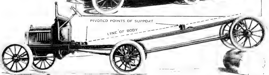
Above and below: The two pivoted points of support in the autoport system distribute the load equally over six wheels. The steering arms of both front and rear wheels are connected by equalizers at each end
